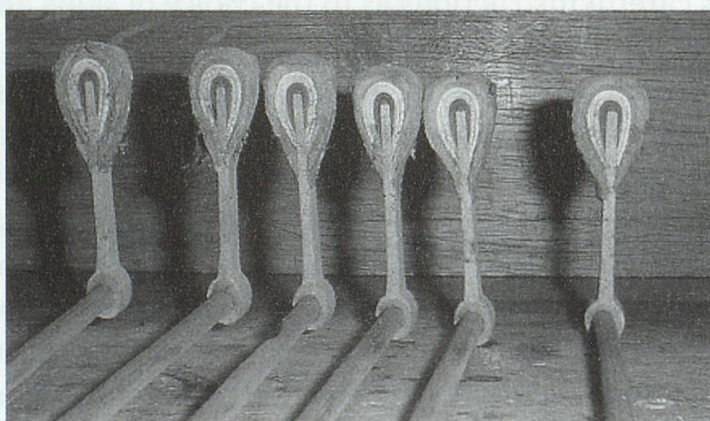
c) Leather-covered hammers by Pape. Note how the asymmetry of the underlayers continues from hammer to hammer; it is probable that the underlayers were applied simultaneously to a block of several hammers.
