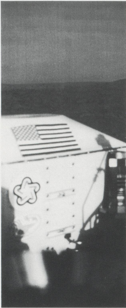
VIEW OF THE CHRYSÉ PLAIN FROM VIKING LANDER I. THE PICTURE WAS TAKEN ON JULY 26, 1976 AT LOCAL MARS TIME OF 7:18 AM.
