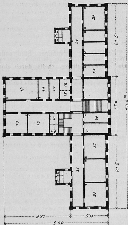
Erdgeschoss.
