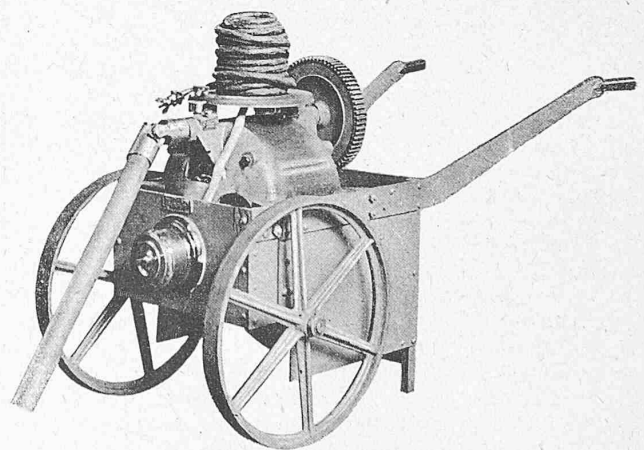
Fig. 5. Transportable Bohrmachine.
