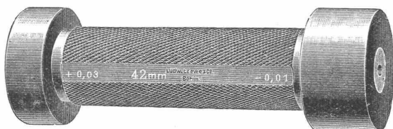
Toleranz-Kaliberdorn.
