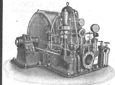
Patent-Freistrah-Turbine. 2500 HP, 300 Meter.
