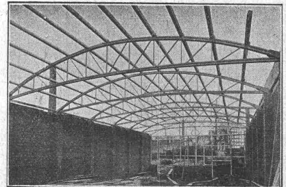
Dachbinder in Holz, System Meltzer.
