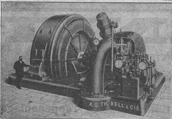
15 000 HP Turbine
