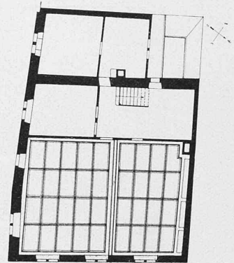
III. Stock. Masstab 1 : 300.
