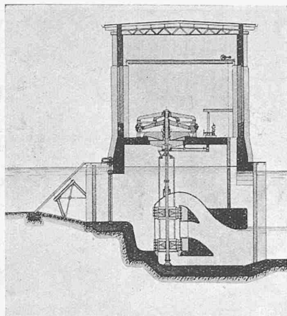
Abb. 16. Kraftwerk Rheinfelden, 1895/98. — 1 : 500. H max 5,0 m; Q = 26 m 3 /sek, N = 1000 PS.
