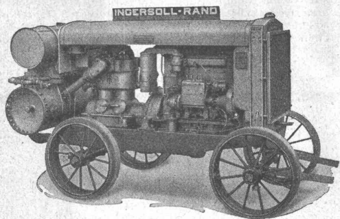
Rohölkompessor 20/26 PS.
