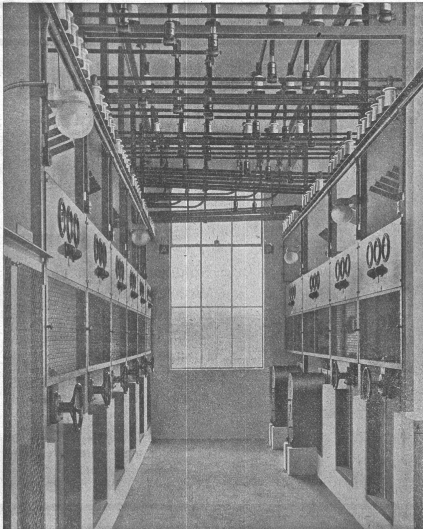
Transformatorstation 6300/3295 V. 50.
