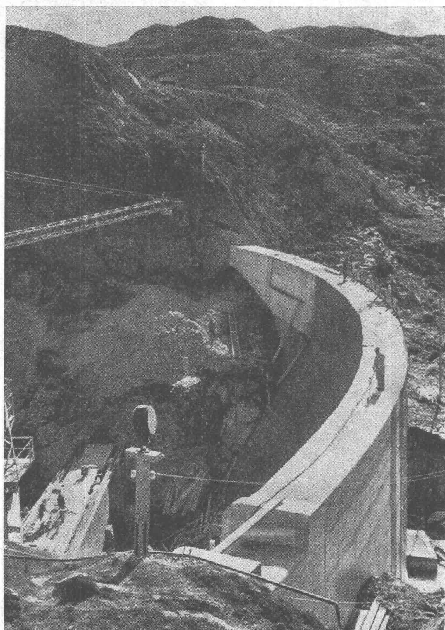
Staumauer Totensee
