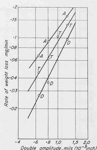
Fig. 11. Rate of weight loss versus Amplitude Material: Plate Steel A 201; Liquid: D Distilled water, T Tap water, A Arkansas river water; Temperature: 80^{\circ}\text{F} ; Frequency 20 000 CPS; Diameter of specimen 0,625 inch
