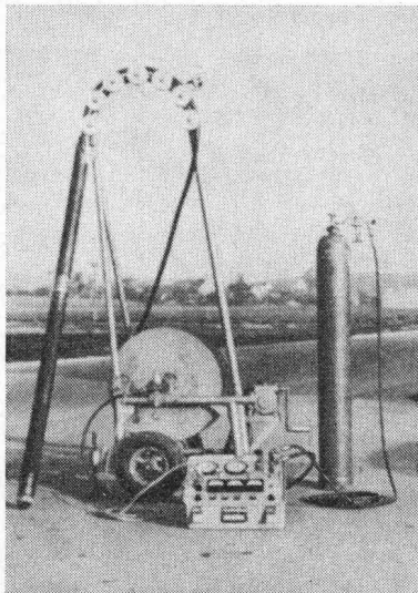
Dilatometer 95
