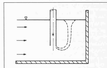
Fig. 9. Formation of an intake vortex in the wake of a vertical pump suction pipe
