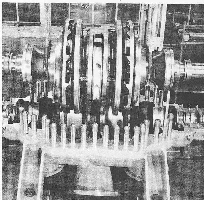
Pumpenrotor (radial)
