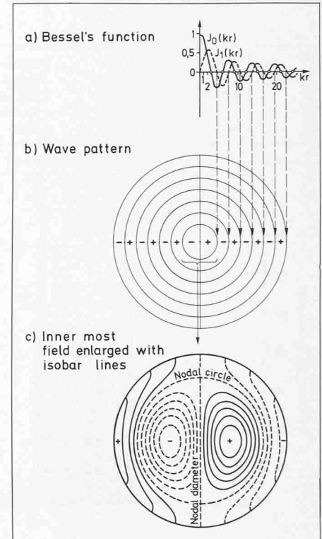
Fig. 3. Bessel's function and wave pattern for a circular gaseous disk (Lamb 1932)
