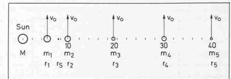
Fig. 2. Parallel-velocity field of the planets held in equilibrium by the gravity of the mass M of the Sun
