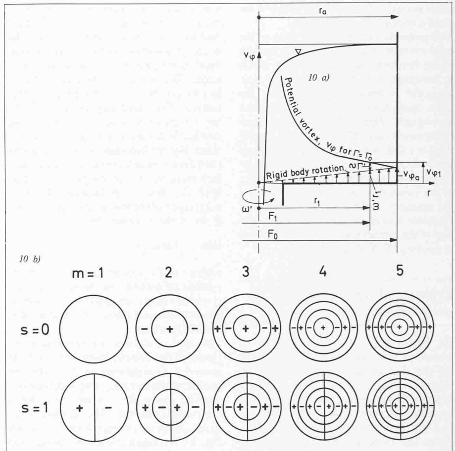
Fig. 10. Derivation of the conservation of circulation in a bath-tub vortex based on the Stokes theorem. a) Transfer of circulation from the outer wall inward due to drain through the central outlet pipe b) Vibration patterns without modal diameter ( s=0 ) and with one nodal diameter ( s=1 )
