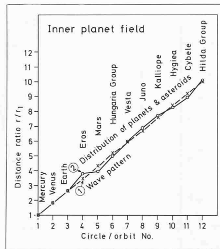
Fig. 5. Distance ratio r/r_1 versus circle/orbit No. for the inner field ( r_1 = distance of the innermost circle/orbit)
