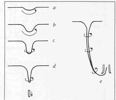
Fig. 7. Stages in development of an air-entraining vortex (Denny)
