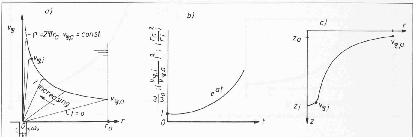
Fig. 8. Transformation from a rigid-body vortex at t = 0 to Rankine vortices with narrowing inner core arising from ventilation of the viscous fluid from the inner core by the axial flow
