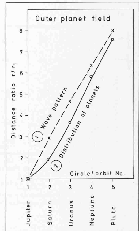
Fig. 6. Distance ratio r/r_1 versus circle/orbit No. for the outer field
