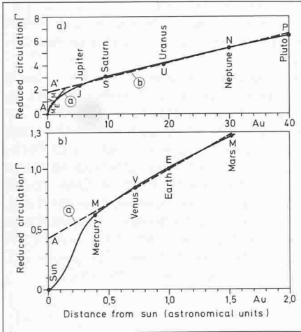
Fig. 1. Circulation \Gamma versus distance r from the Sun for the primordial nebula disk of the solar system a) for the entire system b) for the inner field
