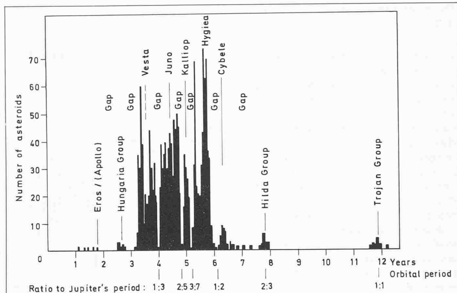
Fig. 4. Distribution density of asteroids with the several Kirkwood gaps
