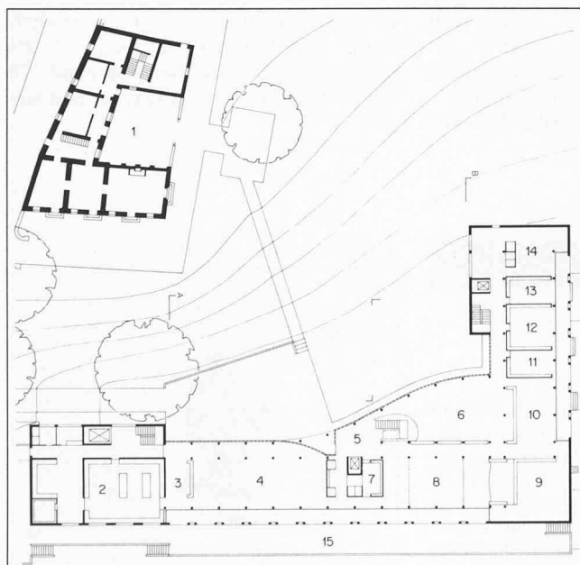
Piano terra 1:700
