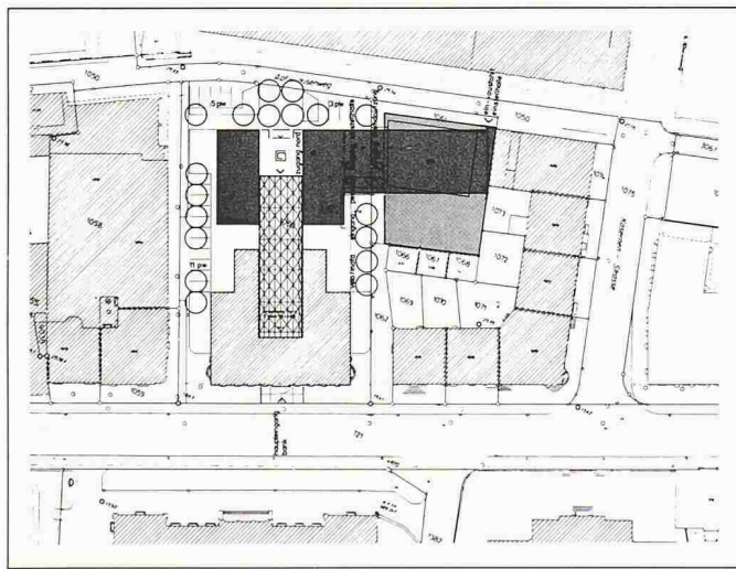
Situationsplan 1:2000
