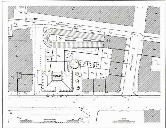
Situationsplan 1:2000
