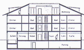
Schnitt Ost-West
