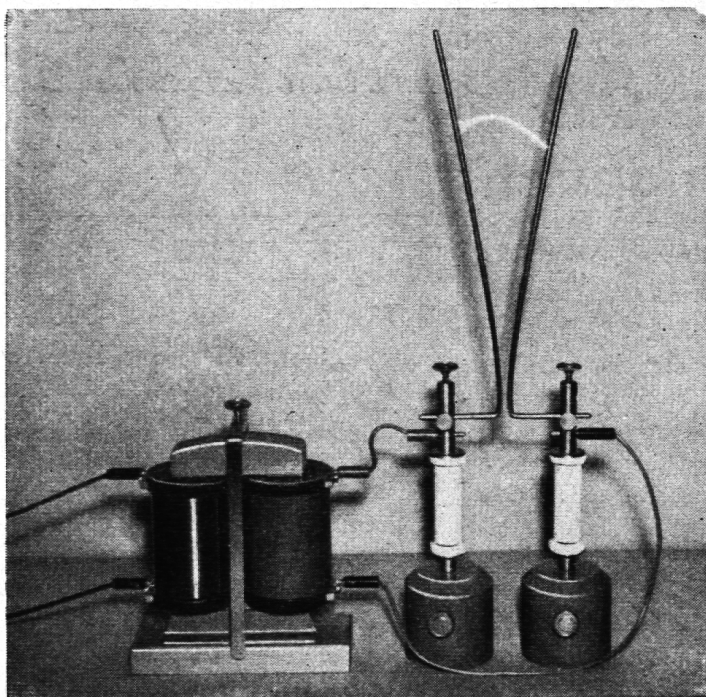
Demonstrationstransformator
