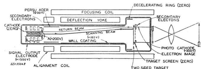
Fig. 9 The Image Orthicon (Schematic Diagram)
