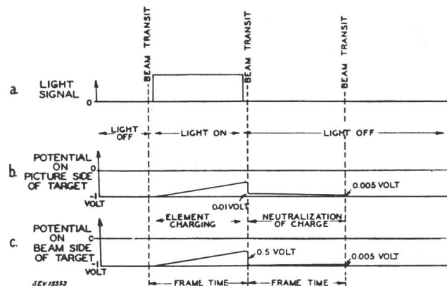
Fig. 13 Potential Variation
