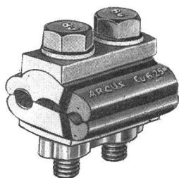
Al-Cu-Klemme
