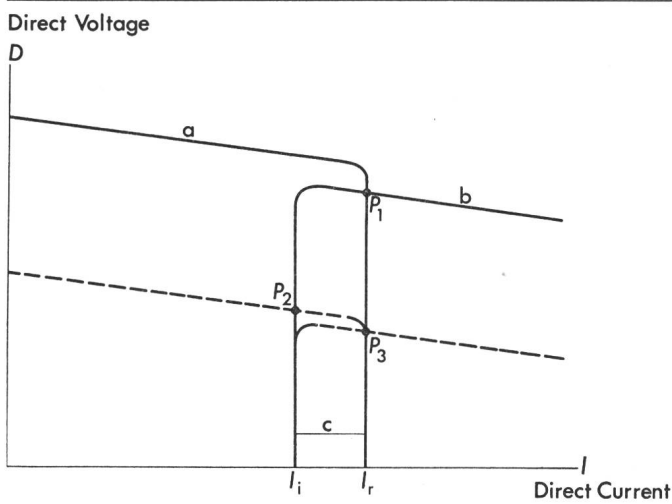
Fig. 3 Control Curve
