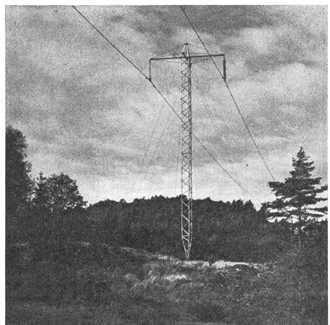
Fig. 4 HVDC Overhead line
