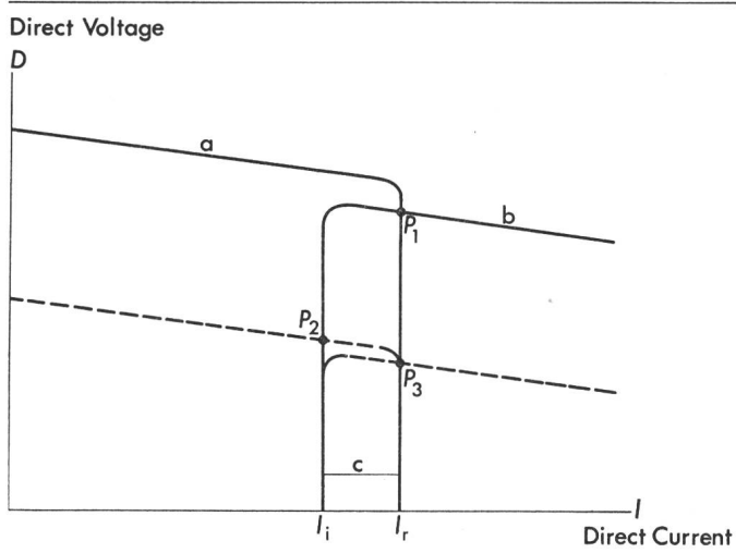
Fig. 3 Control Curve
