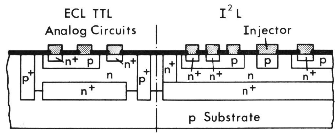
Fig. 3 Possibility of combining the bipolar I 2 L technique with conventionally isolated transistors on one chip
