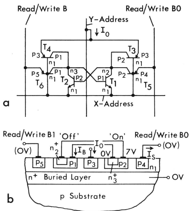
Fig. 14 Equivalent circuit diagram and cross-section of the structure of an injection-coupled RAM-cell [18]
