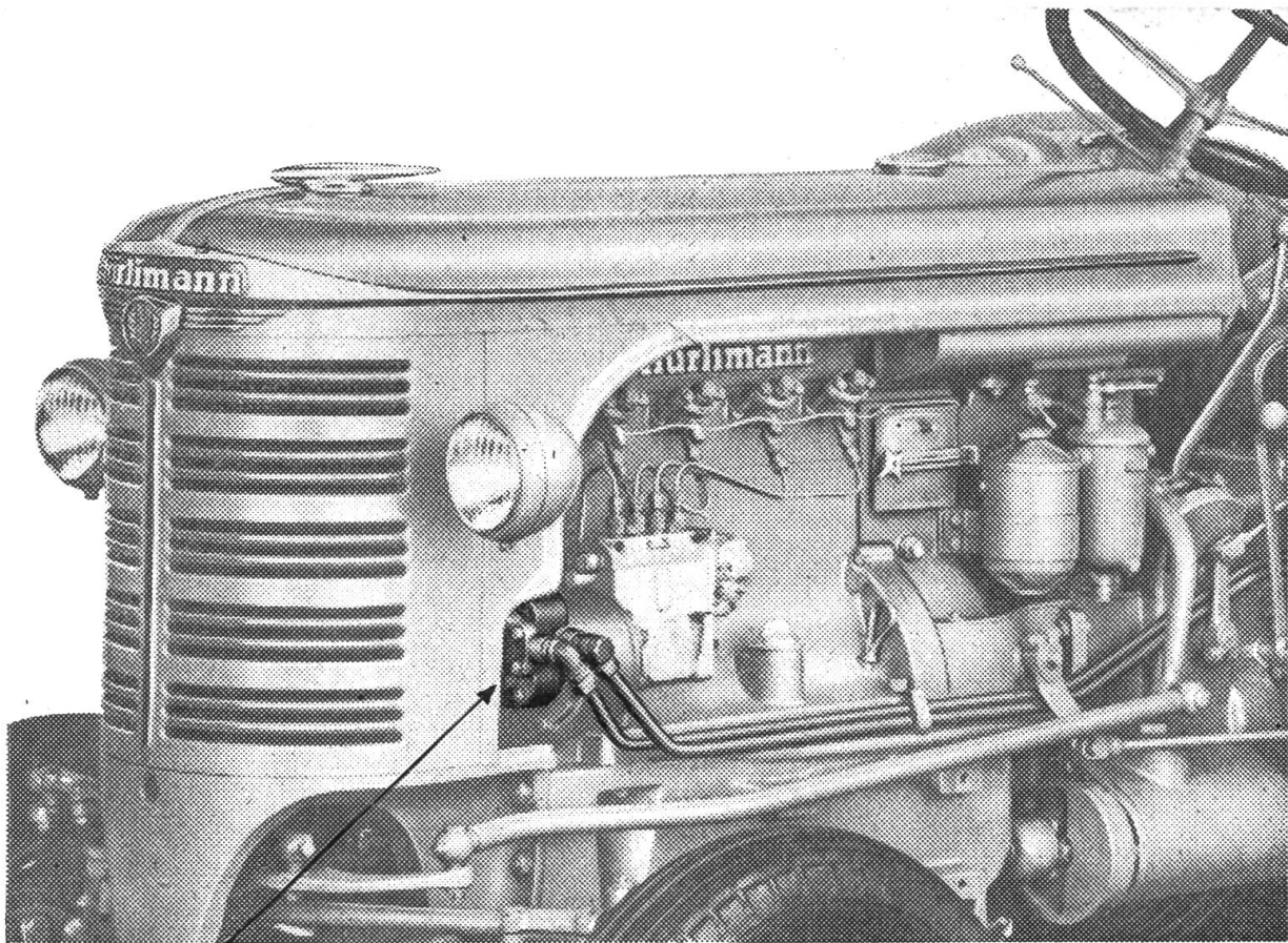
Hydraulikpumpe
