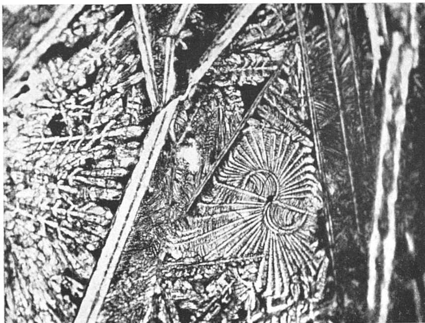
Photo Nr. 6. Arborescent skeletal augite growth, within lamellae of serpentine minerals. Diabase ("Octahedral" type) of Punta Trinidad. Gorgona. Approx. Enlarg. 120 \times .
