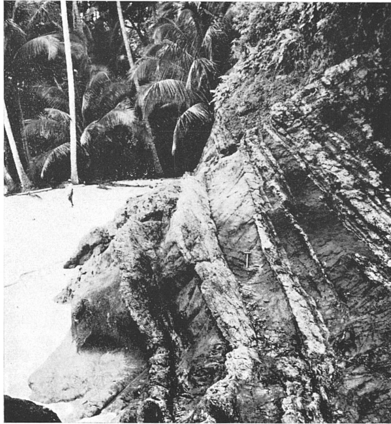
Photo Nr. 3. Banded Upper Eocene of Gorgonilla, consisting of an alternation of tuffaceous sandstones and siliceous shales.
