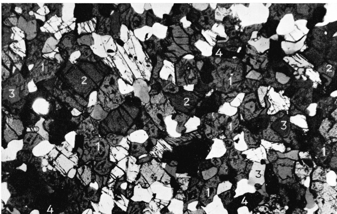
Fig. 1. Amphibolite containing isotropic unknown mineral N of Belihun, Sierra Leone. Thin section 40\times . N // . 1 = dixeyite; 2 = hornblende; 3 = quartz; 4 = magnetite.
