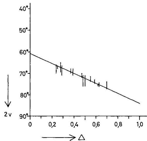
Fig. 4. 2V /triclinicity ( \Delta ) correlation diagram. (Specimen No. 1739.) The ranges of the observed variations in 2V are shown as lines above the corresponding triclinicity values, measured by X-rays on the same samples. The error in triclinicity is \pm 0.03 .
