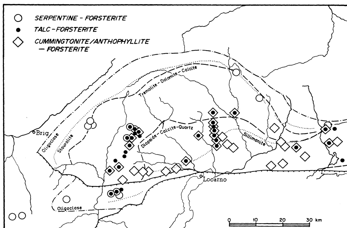
Fig. 4. Regional occurrence of the assemblages serpentine + olivine, talc + olivine and cumingtonite/anthophyllite + olivine in the Lepontine Alps.
