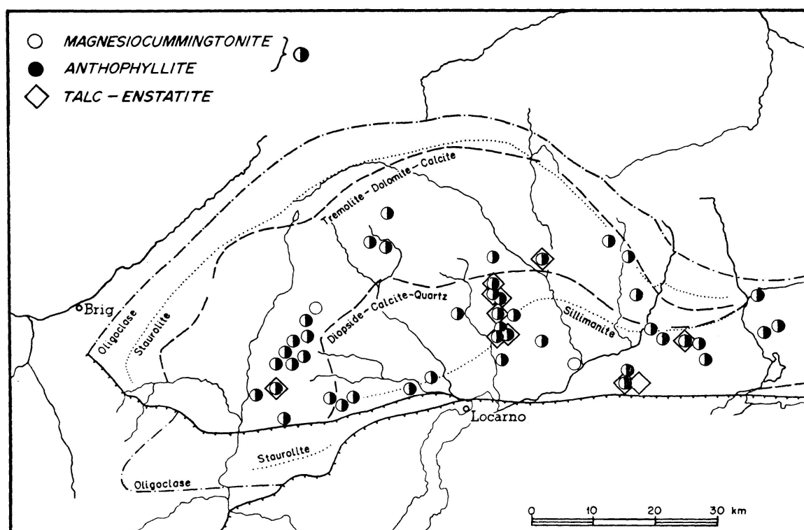
Fig. 5. Regional occurrence of magnesioCumingtonite, anthophyllite, and talc + enstatite in the Lepontine Alps.
