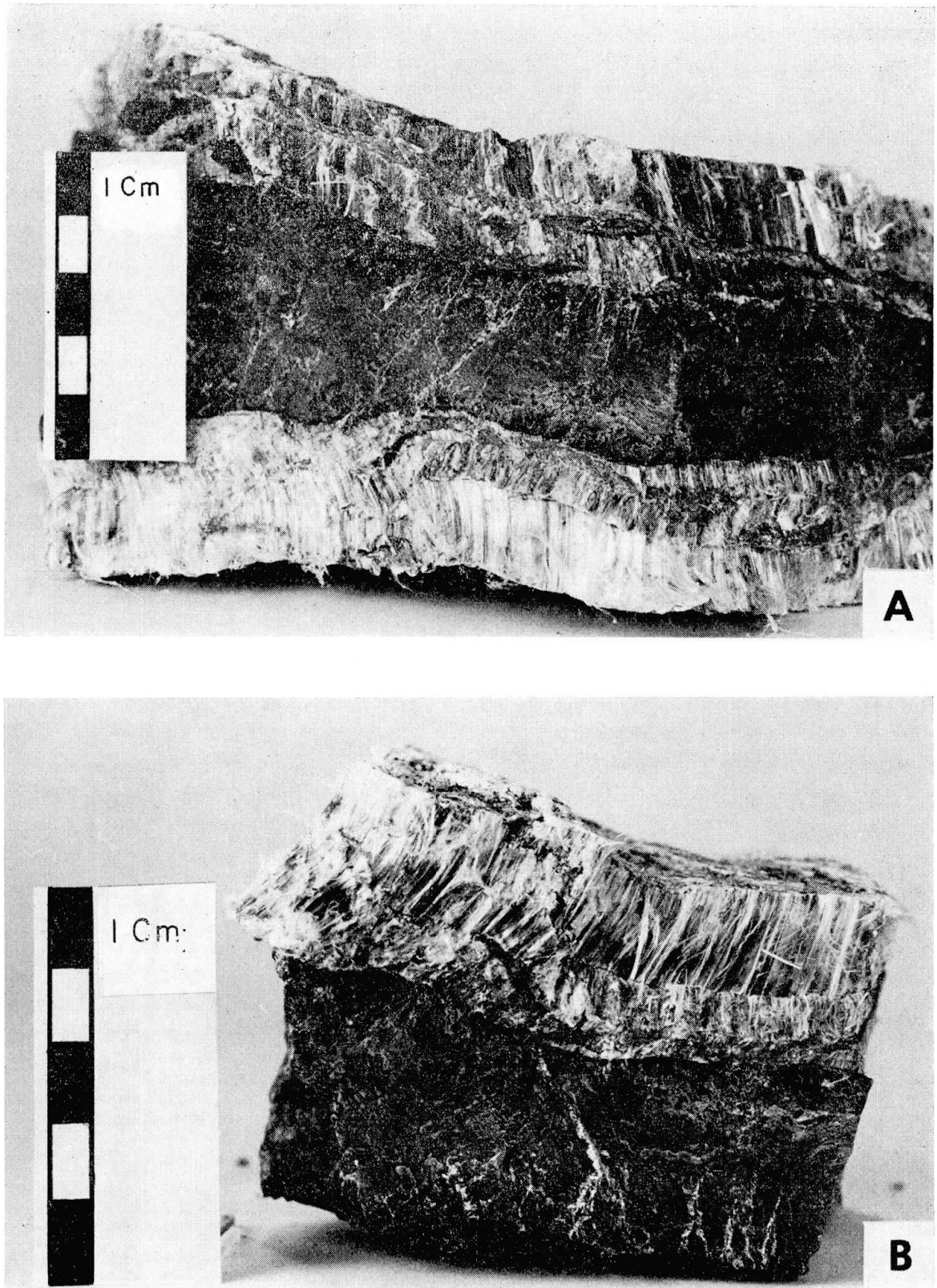
Fig. 8. Composite veins ("type c") of chrysotile fibres from the region of Thetford Mines. The veins are formed by a combination of simple veins and veins with a median suture. In both figures A and B, one can see examples of serpentinite inclusions along the median suture of some veins.
