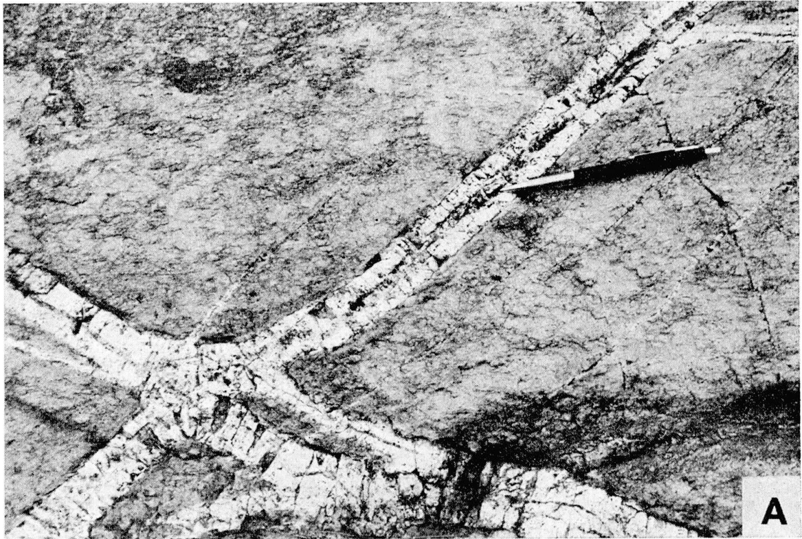
Fig. 2a. Tectonite fabric in serpentized harzburgite at Vimy Ridge. The porphyroclasts of enstatite are in relief and set into a finer-grained matrix of olivine which is pervasively serpentinized. The foliation is parallel to the pencil used as a scale and to the bisectrix of the acute angle of the cross formed by the asbestos veins.
