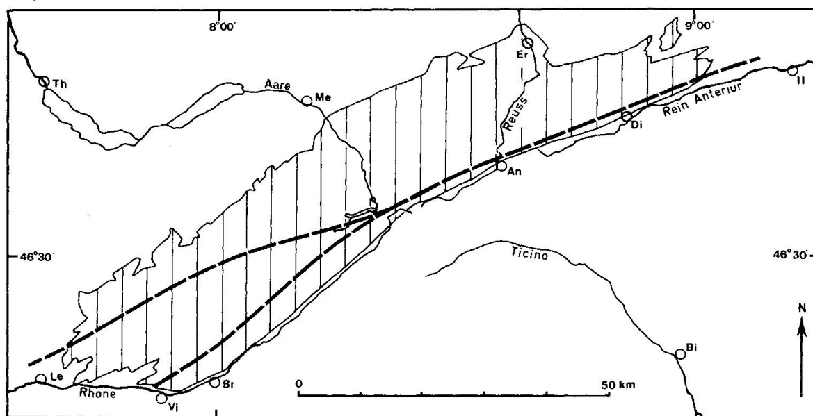
Fig. 1 Sketch map showing the extent of the Rhine-Rhone zone (dashed). An Andermatt, Bi Biasca, Br Brig, Di Disentis, Er Erstfeld, Il Ilanz, Le Leuk, Me Meiringen, Th Thun, Vi Visp. Vertical hatching: crystalline rocks of the Aar massif.
