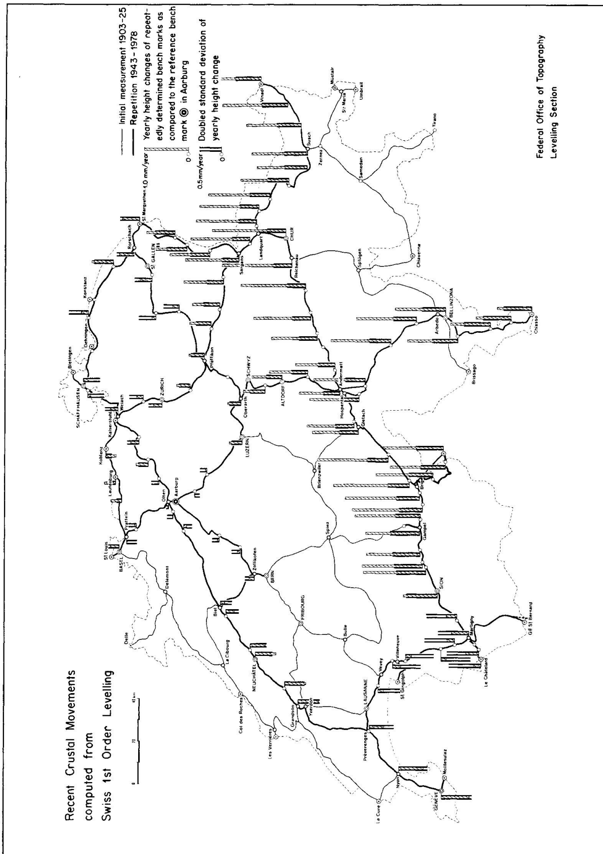
Fig. 2 Rates of vertical crustal movements in Switzerland derived from re-observed precise levelling lines 1903-1925 and 1943-1979. After GÜBLER, 1979.
