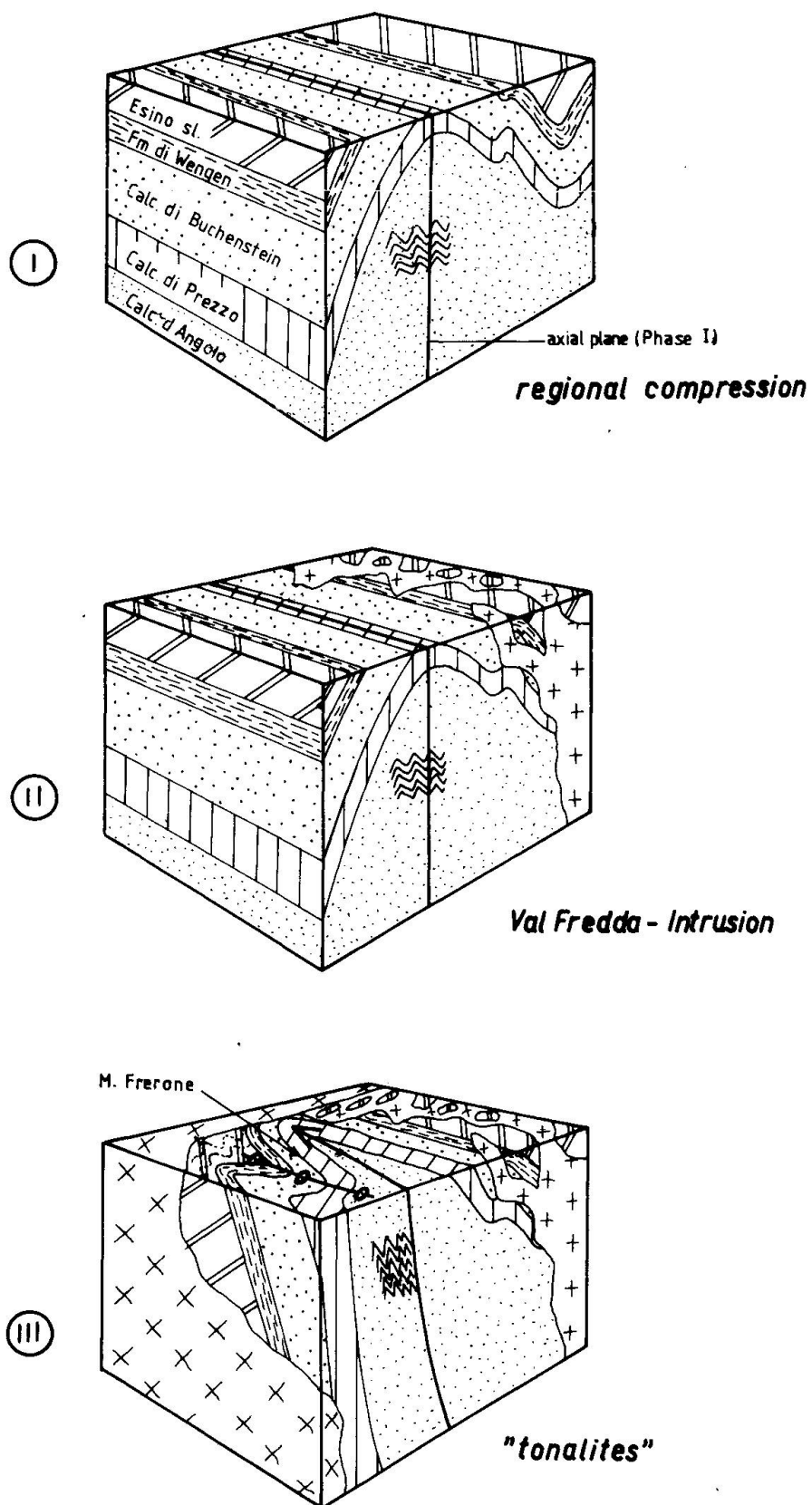
Fig. 6 Tectonic development of the M. Frerone area.
