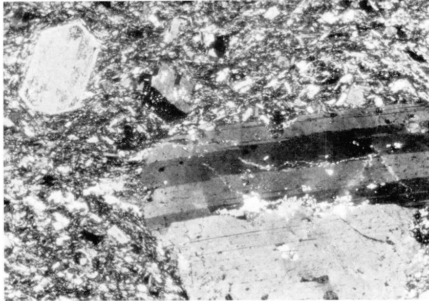
Fig. 13 Keratophyre. Phenocrysts of albite showing normal twinning, embedded in a felsitic matrix. Inclusion zoning is also seen. (L = 3.27 mm, with analyser)
