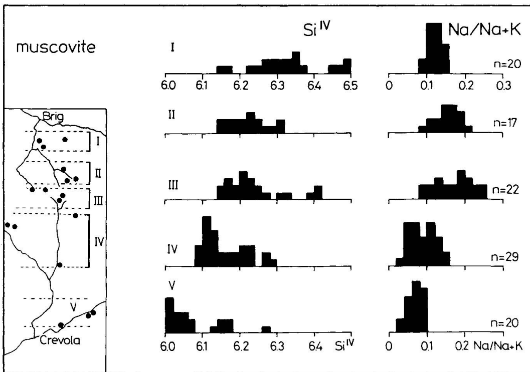
Fig. 10 Regional variation of muscovite composition as a function of increasing metamorphic grade: variation of Si^{IV} and Na/Na+K .
