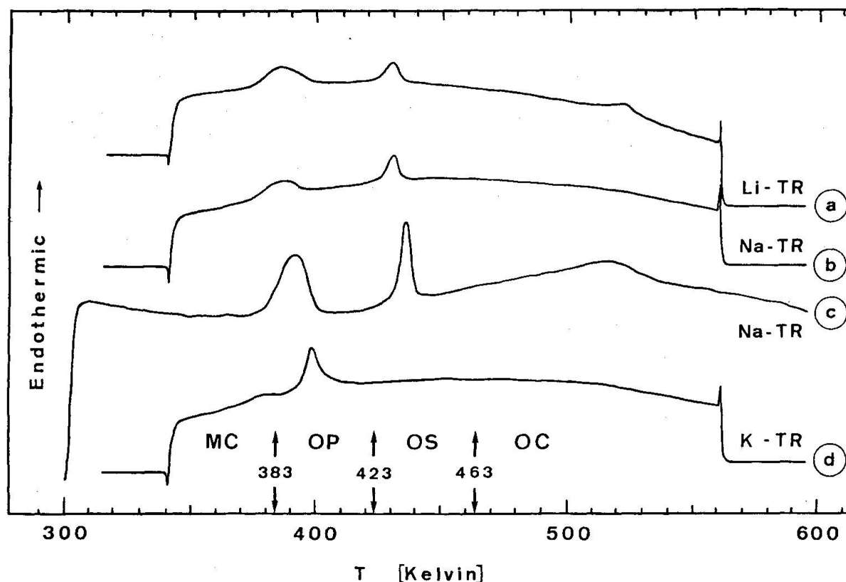
Figure 4 Tracings of the DSC scans for synthetic alkali- \text{WO}_4 fluxgrown tridymites over narrow temperature ranges. Scans a, b and d are first heating-scans from 340 to 560 K on the lithium, sodium and potassium fluxed preparations. Same instrument settings as in Figure 1 were used. The sample weights were about 24 mg for Li-TR and 30 mg for Na-TR and K-TR respectively. Scan c was made from 300 to 600 K on the DSC-2C, and revealed the 517 K peak in Na-TR.
