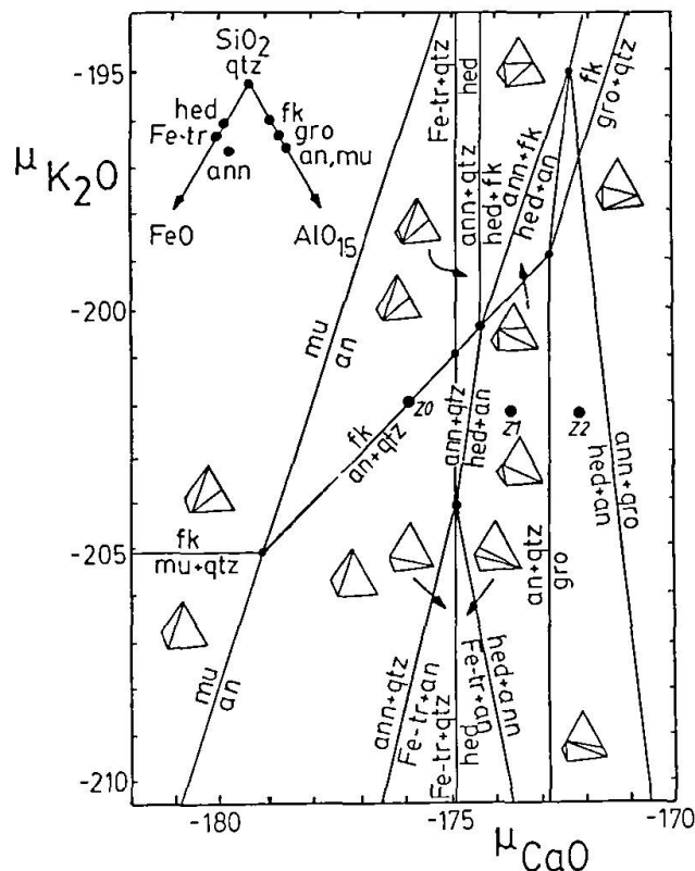
Fig. 8 (after VAN MARCKE DE LUMMEN and VERKAEREN, 1986). \mu_{CaO}-\mu_{K2O} (kcal/mole) diagram in the system K_2O-CaO-FeO-Al_2O_3-SiO_2-H_2O ( Na_2O is considered as an accessory component) with the minerals: quartz (qtz), anorthite (an), K-feldspar (Ksp), muscovite (mu), annite (ann), Fe-tremolite (Fe-Tr), hedenbergite (hed) and grossular (gro). P_s = P_f = 2 kb, T = 600^\circ C , X_{H_2O} = 1.0 . ZO, Z1, Z2 refer to the different zones observed in endoskarns (see Tab. 1).
