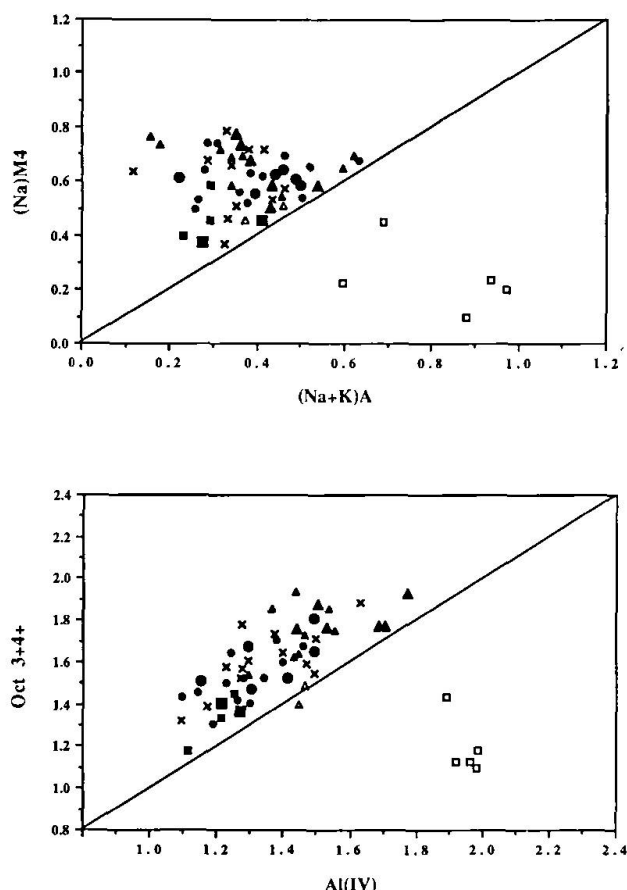
Fig. 5 Formula proportion diagrams (LAIRD and ALBEE, 1981) of amphiboles from the Korälpe and Saualpe eclogites. Symbols as in Fig. 2 with smaller symbols representing amphiboles (I) and larger symbols denoting poikiloblastic amphiboles (II). Crosses represent amphibole inclusions in garnet, omphacite, kyanite and zoisite. Note that amphiboles (III) from strongly overprinted eclogites (open squares) clearly plot in the range of low pressure series mafic schists.
