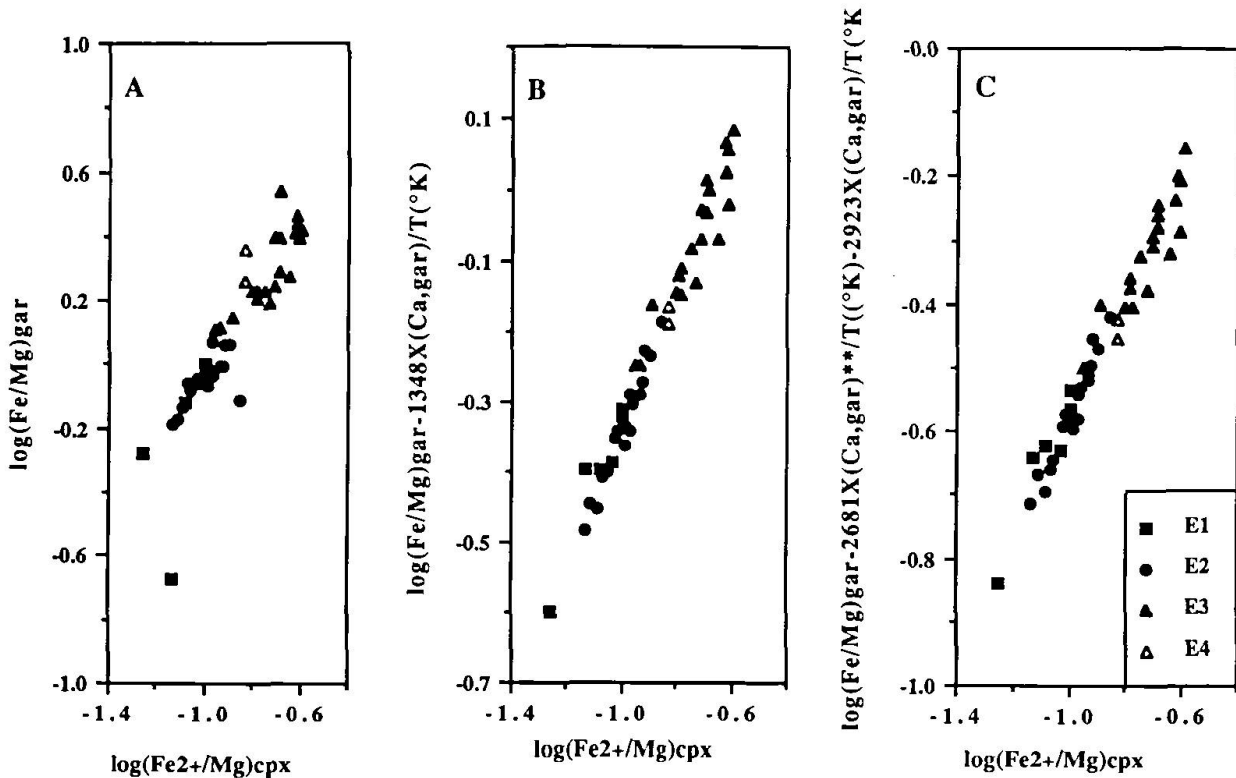
Fig. 6 (A) Logarithmic distribution of \text{Fe}^{2+}/\text{Mg} between garnets and clinopyroxenes from the Koralpe and Sau-alpe eclogites (B). The same data as in (A), corrected for X_{\text{Ca}}^{\text{Gar}} (B) after ELLIS and GREEN (1979), resp. (C) after KROGH (1988). Asteriks denote power of two.
