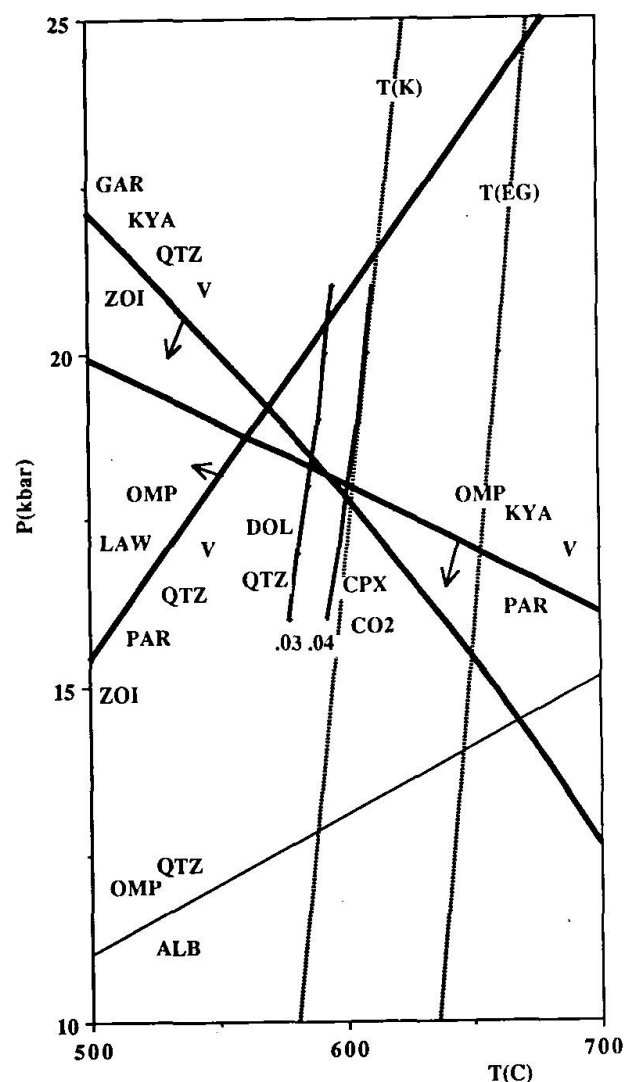
Fig. 7 Estimated peak metamorphic conditions for Koralpe and Saualpe type (2) eclogites. Mineral equilibria calculated from data of POWELL and HOLLAND (1988) using the following activities: a_{\text{gar}} = 0.310 , a_{\text{gross}} = 0.020 , a_{\text{par}} = 0.820 , a_{\text{zoi}} = 0.900 , a_{\text{jad}} = 0.610 , a_{\text{dol}} = 0.900 . Iso- K_D -lines T(EG) and T(K) for \text{Fe}^{2+}/\text{Mg} distribution between garnet and clinopyroxene calculated after ELLIS and GREEN (1979), resp. after KROGH (1988). Arrows indicate displacement due to a_{\text{H}_2\text{O}} < 1.0 .
