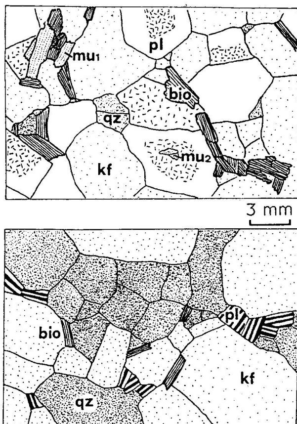
Fig. 5 Fabric patterns and mineral compositions of the monzogranite from Klein-Zadel (Hauptgranit) and the leuco-monzogranite from Meißen (Riesensteingranit). Abbreviations as in figure 2. Note the occurrence of magmatic (mu1) and late- to post-magmatic (mu2) muscovite.
