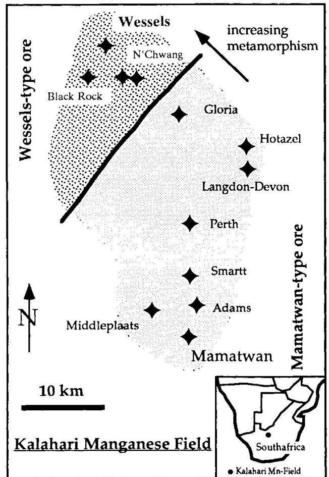
Fig. 1 Sketch map of the Kalahari Manganese Field.
