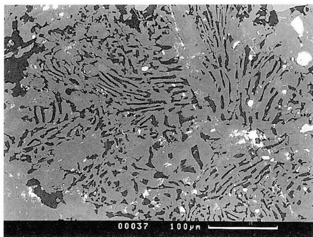
Fig. 4 Back-scattered electron (BSE) image of sodic diopside (up to 15 mole % of Jd; pale gray) and oligoclase ( \text{Ab}_{90}\text{An}_{10} – \text{Ab}_{80}\text{An}_{20} ; black) symplectite after omphacite (sample Ua36, Unteralptal).
