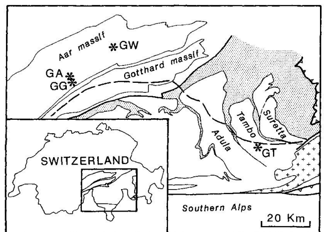
Fig. 1 Location of the metagranite shear zones. GT: Truzzo granite (Tambo nappe); GG: Grimsel granodiorite (Aar massif); GA: Aar Granite (Aar massif); GW: Wassen granite (Aar massif). The dashed line corresponds to the greenschist facies – amphibolite facies boundary.
