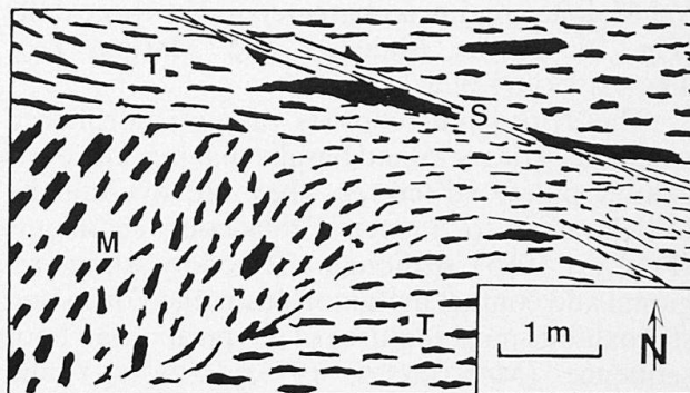
Fig. 4 Outcrop sketch of near-vertical gabbro structures above Alpe Lagazuolo (Swiss grid coordinates: 782.900/129.500). Magmatic flow textures (M) occur in boudins surrounded by tectonic flaser structures (T) which are cut by later shear zones (S).
