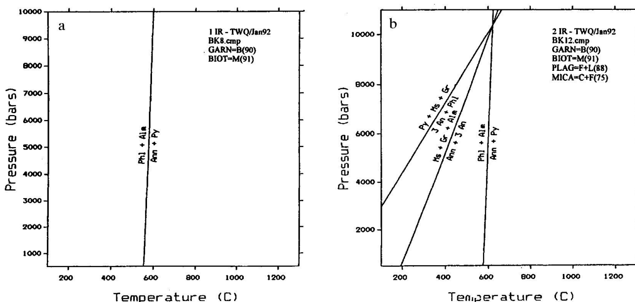
Fig. 9 Representative examples of thermobarometric results obtained from the Tweek program. (a) BK8: Garnet-biotite thermometry, and (b) BK12: garnet-biotite-muscovite-plagioclase thermobarometry.
