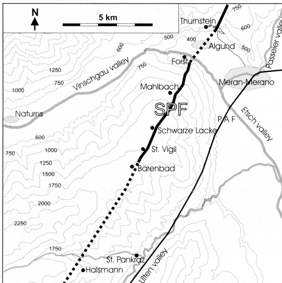
Fig. 2 Location of Southern Pässeier fault (SPF). Continuous thick line shows the distribution of cataclastic to mylonitic rocks of the SPF in the field. Dotted line traces the SPF as recognised from the satellite image analysis and the radiometric age distribution pattern. The Periadriatic fault (PAF) is located to the east of the SPF.
