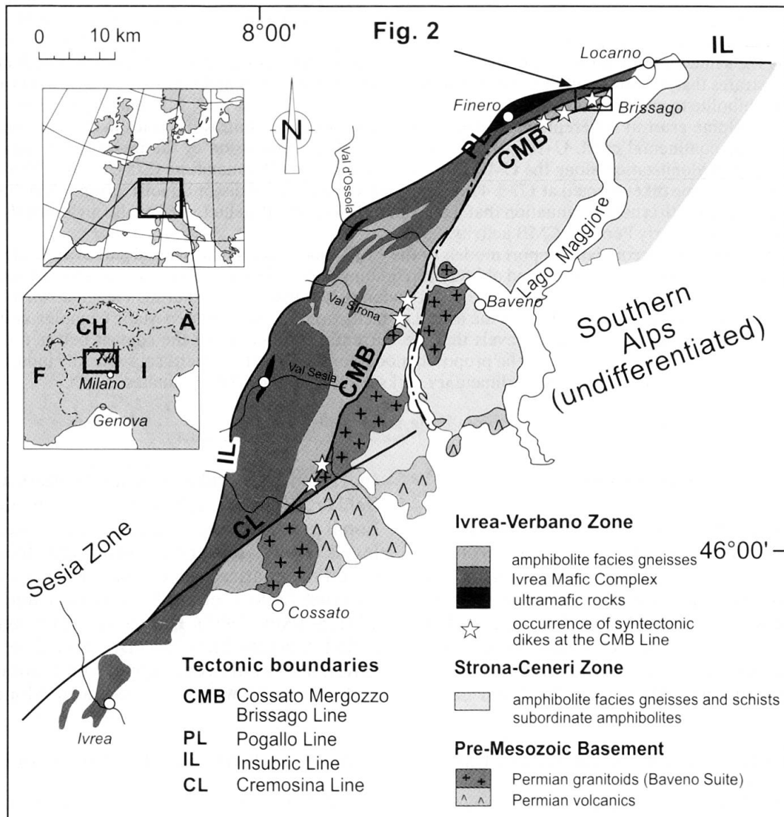
Fig. 1 Sketch map of the western part of the southern Alpine basement units modified from ZINGG et al. (1990). Framed area is shown in detail in Figure 2.
