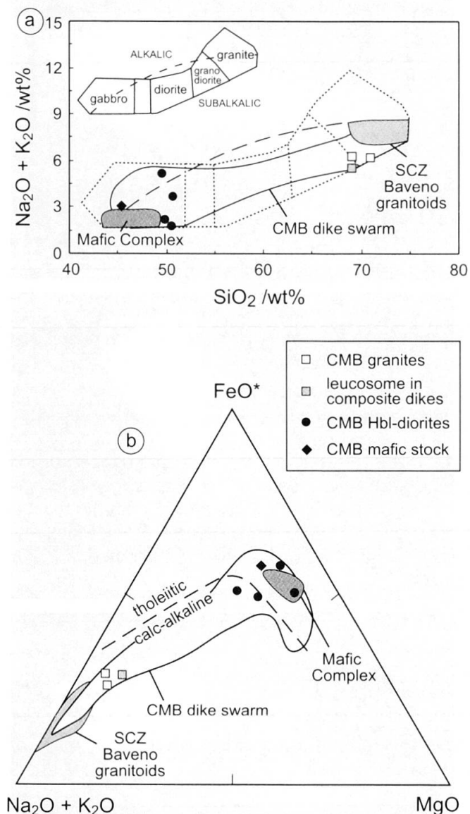
Fig. 7 (a) Total alkali vs. SiO 2 (TAS) plot with classification of subalkalic plutonic rocks after WILSON (1989). Note that pyroxene-free CMB hornblende-dioritic dikes plot in the gabbro field due to high modal amounts of primary hornblende and biotite that are low in SiO 2 with respect to pyroxene. These low-SiO 2 hornblende-dioritic dikes (filled circles and diamond) are therefore interpreted as being close to one end-member composition of the CMB dike swarm. (b) AFM ternary plot with tholeiitic to calc-alkaline division. Data defining fields of Mafic Complex, CMB dike swarm and Baveno granitoids in (a) and (b) are from BORIANI et al. (1974), GIOBBI ORIGONI et al. (1988), PINARELLI et al. (1988), BORIANI et al. (1992), BORIANI et al. (1995), SINIGOI et al. (1994) and ZURBRIGGEN (1996).
