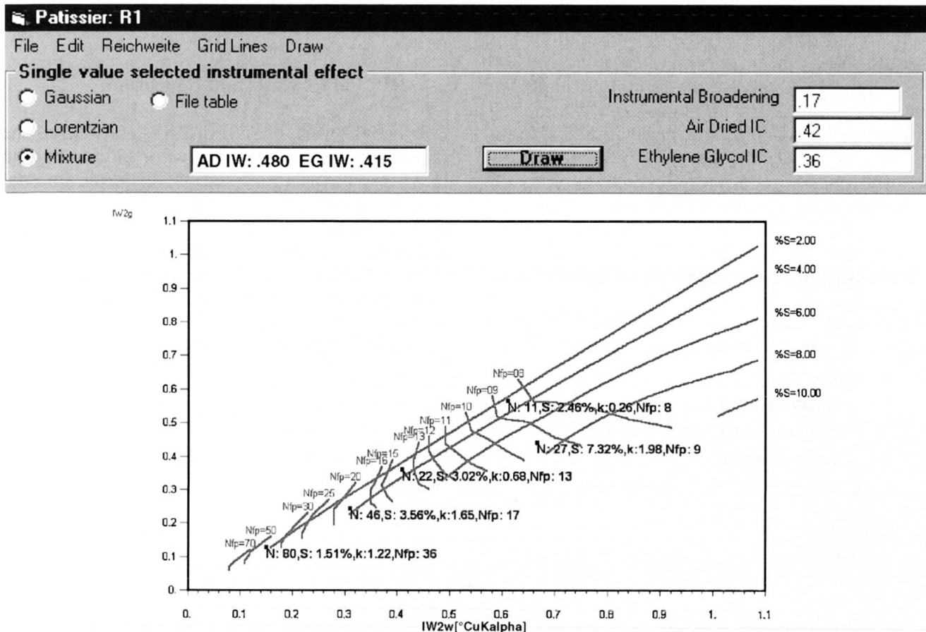
Fig. 4 Window of the program "PATISSIER" with an example including the correction for an instrumental broadening of 0.17 °Δ2θ CuKα and other five examples obtain by clicking directly on the window.
