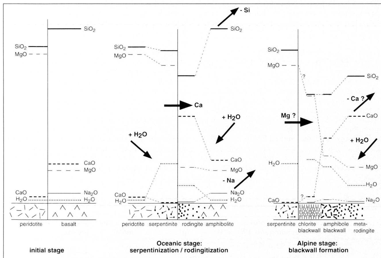
Fig. 15 Schematic sketch showing the mobility of some important major elements from the initial stage to the stage of serpentinitization/rodingitization (oceanic stage) and the process of blackwall formation (Alpine stage).
