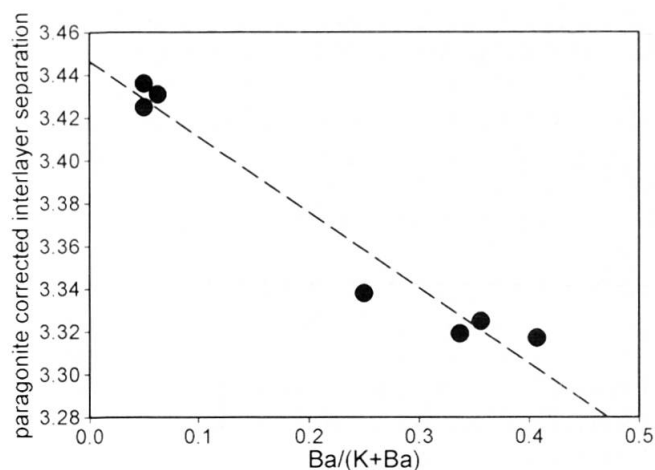
Fig. 7 Influence of Ba/(K+Ba) on the interlayer separation (IS) corrected for the effect of Na (paragonite). The dashed line represents a linear regression through the data points: IS (\text{Å}) = 3.446 - 0.3531 \times Ba/(K+Ba) , ( r^2 = 0.958 ).
