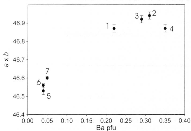
Fig. 8 Ba^{2+} in dioctahedral micas is mainly charge balanced by the substitutions Ba + [^{VI}]Al \leftrightarrow K + [^{VI}]Si and Ba + [^{VI}](Mg, Fe^{2+}) \leftrightarrow K + [^{VI}]Al . Both types of substitution cause a lateral expansion of the sheets, observed as an increase of the a and b cell dimensions. The (001) surface area is determined by a \times b (\text{Å}^2) .
